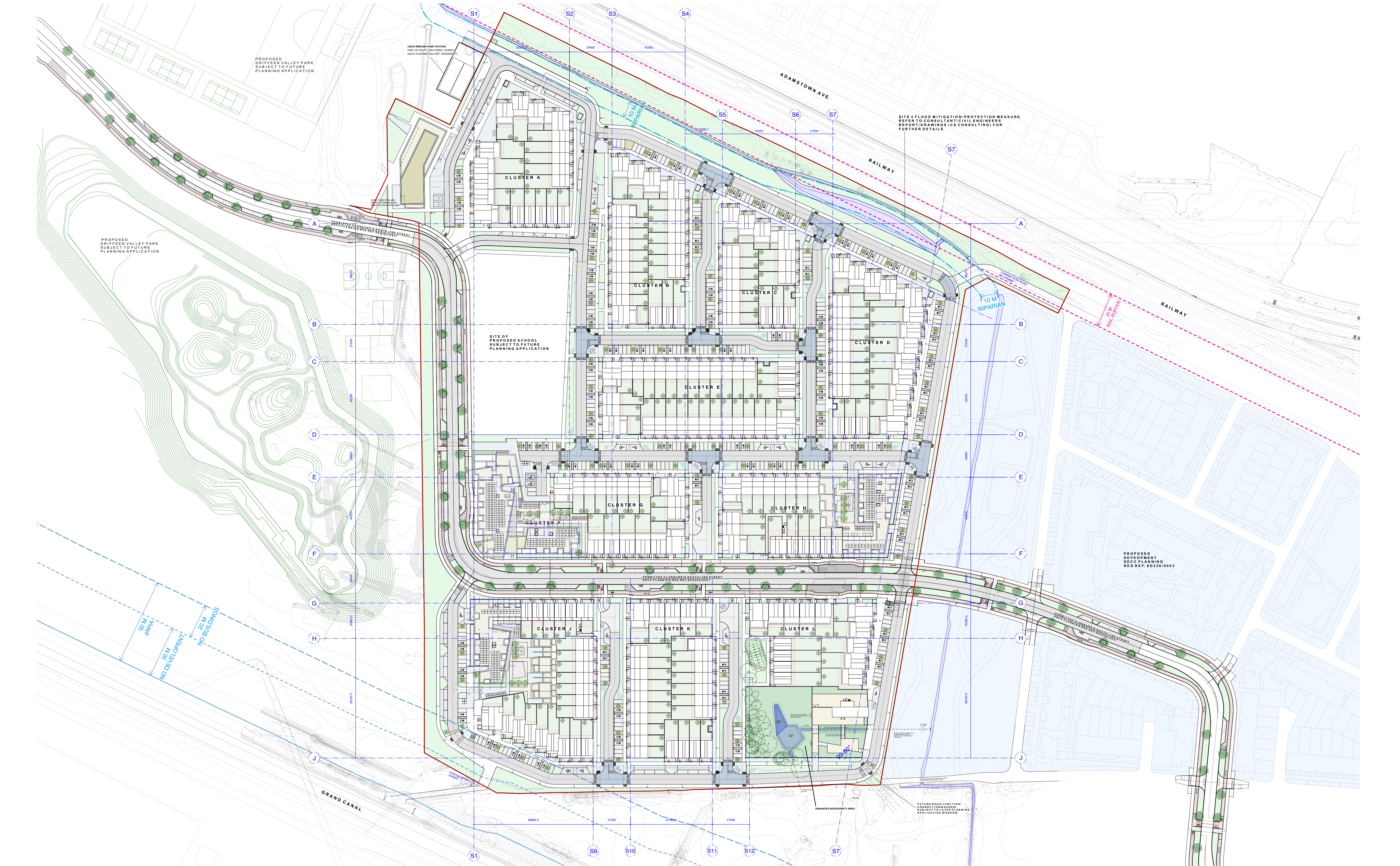
SITE LAYOUT PLAN 1:1000 @ A1
